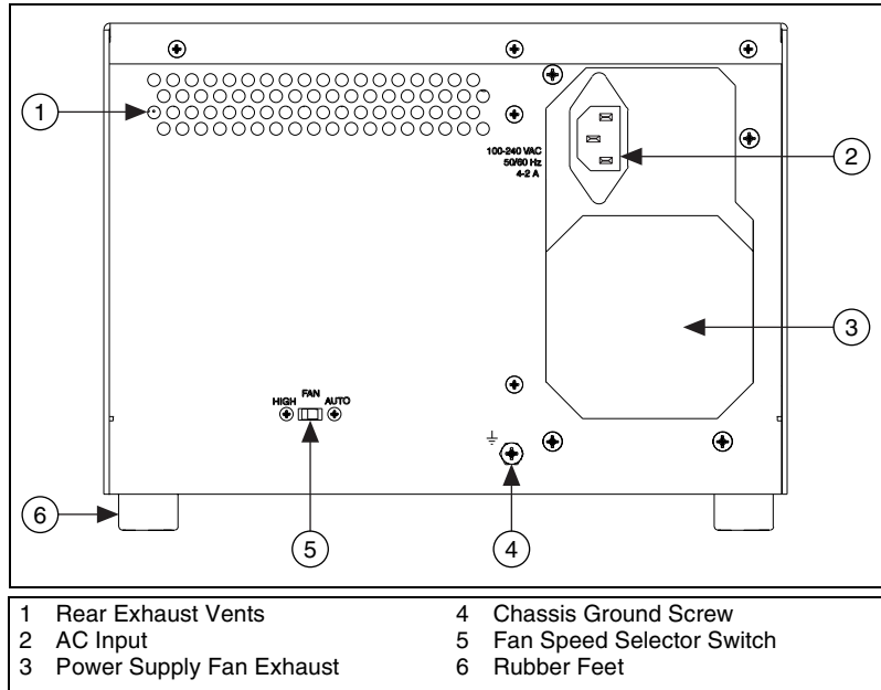
Figure 1-2. Rear View of the PXI-1031 Chassis
