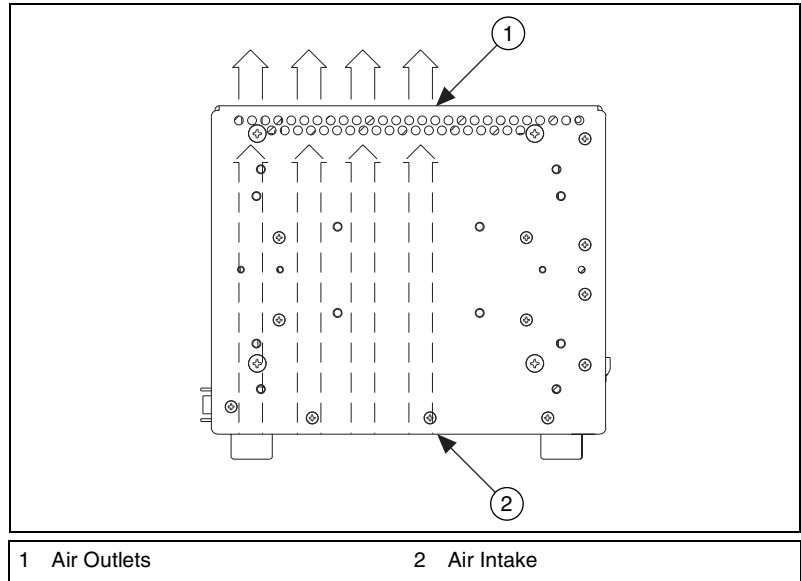
Figure 2-1. PXI-1031 Module Cooling Airflow Side View
