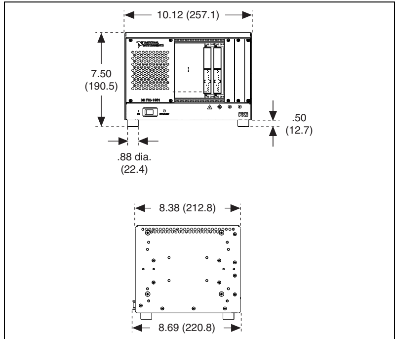
Figure A-1. PXI-1031 Dimensions (Front and Side) in Inches (mm)
