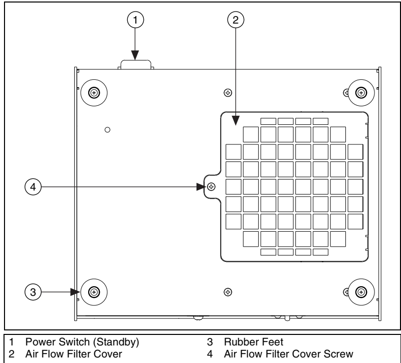
Figure 1-3. Bottom View of PXI-1031 Chassis
