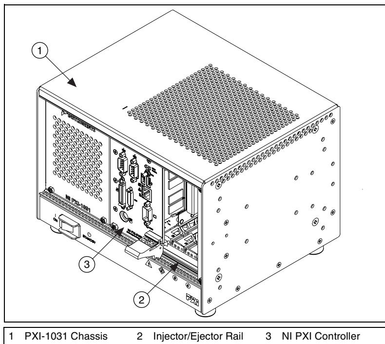
Figure 2-3. NI PXI Controller Installed in a PXI-1031 Chassis
