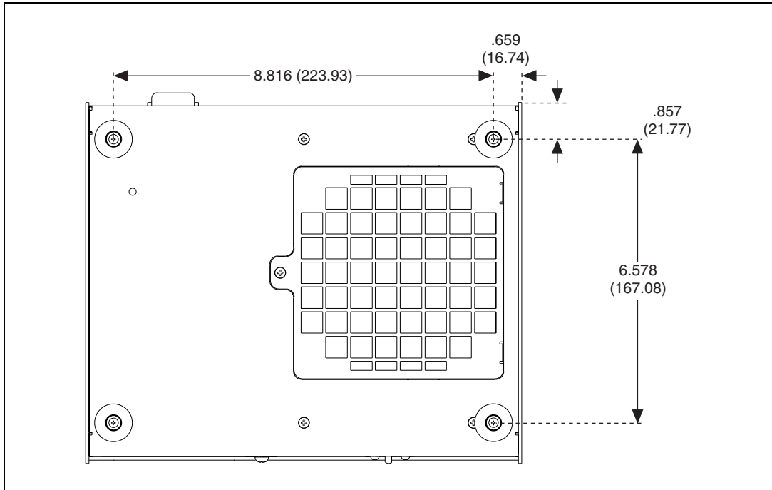
Figure A-2. PXI-1031 Dimensions (Bottom) in Inches (mm)
