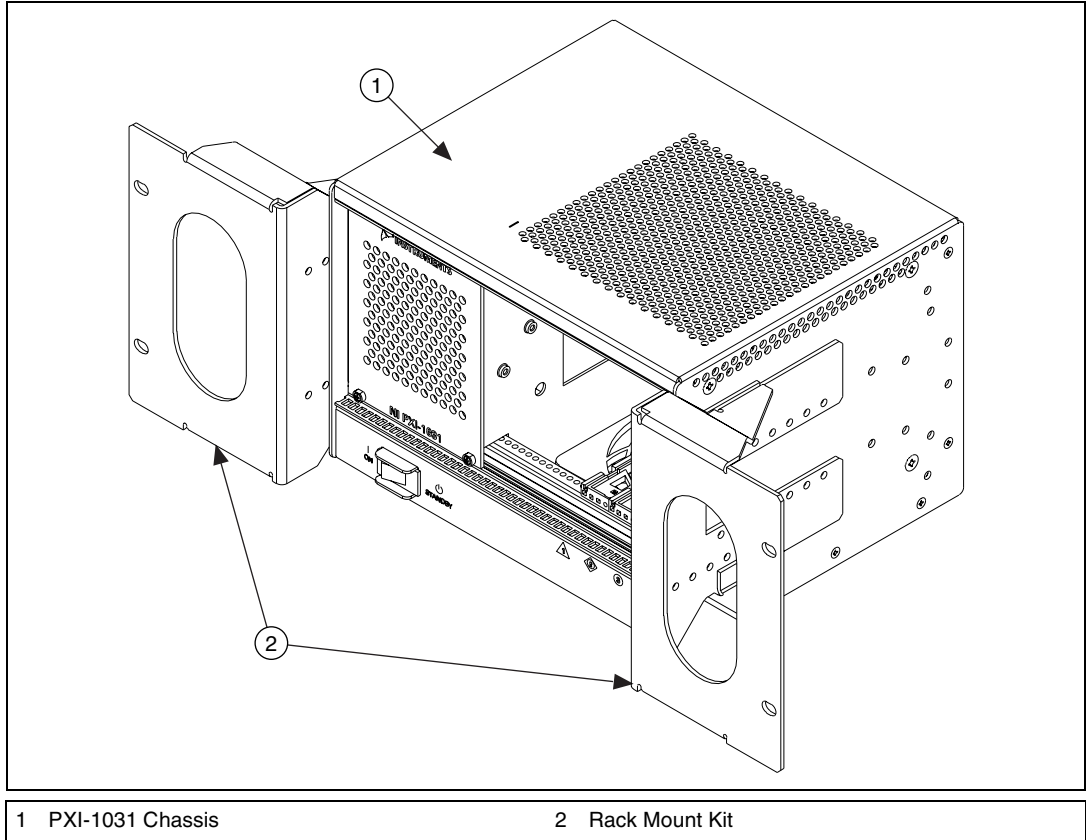
Figure A-3. PXI-1031 Rack Mount Kit Components
